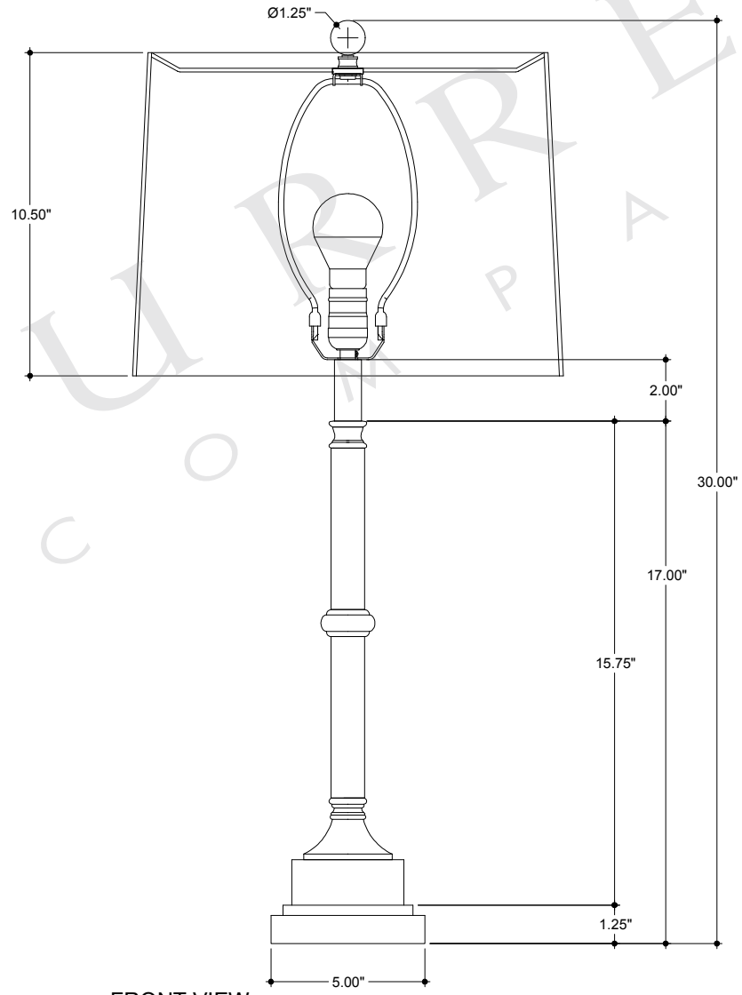
FRONT VIEW
