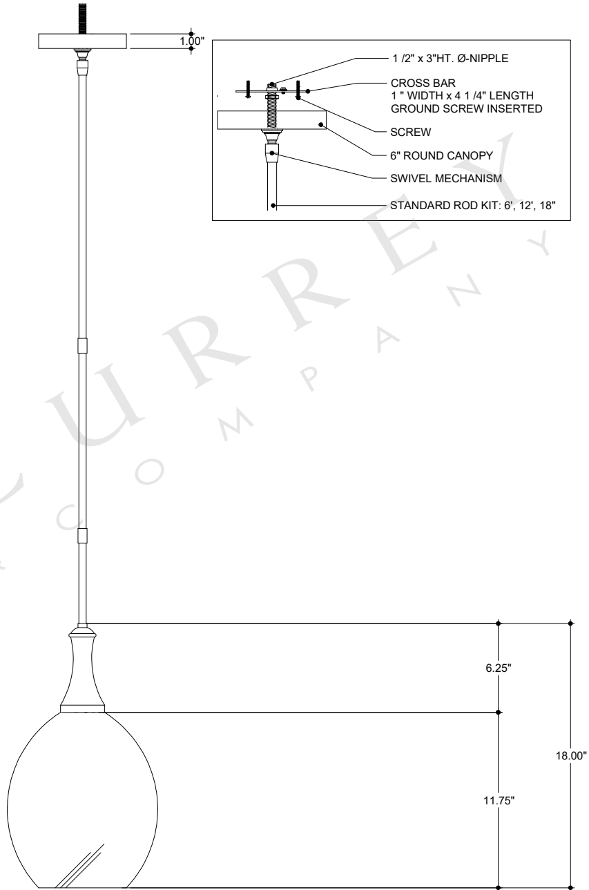
FRONT VIEW
