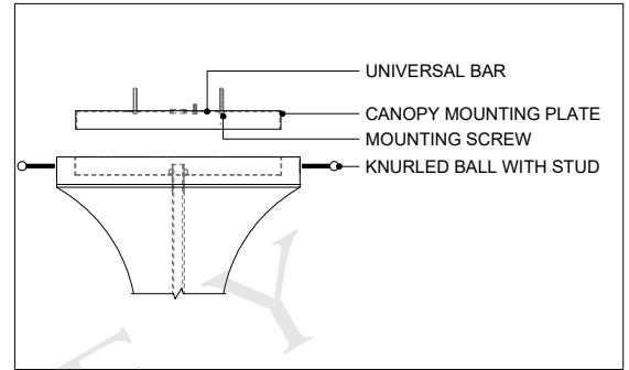
CANOPY DETAIL
