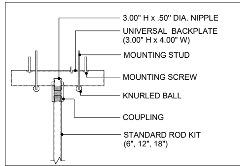
CANOPY DETAIL
