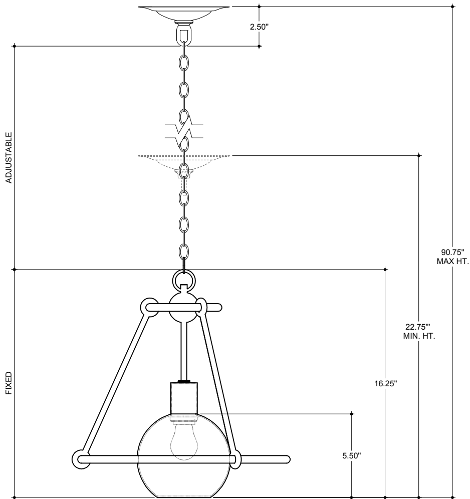
FRONT VIEW
