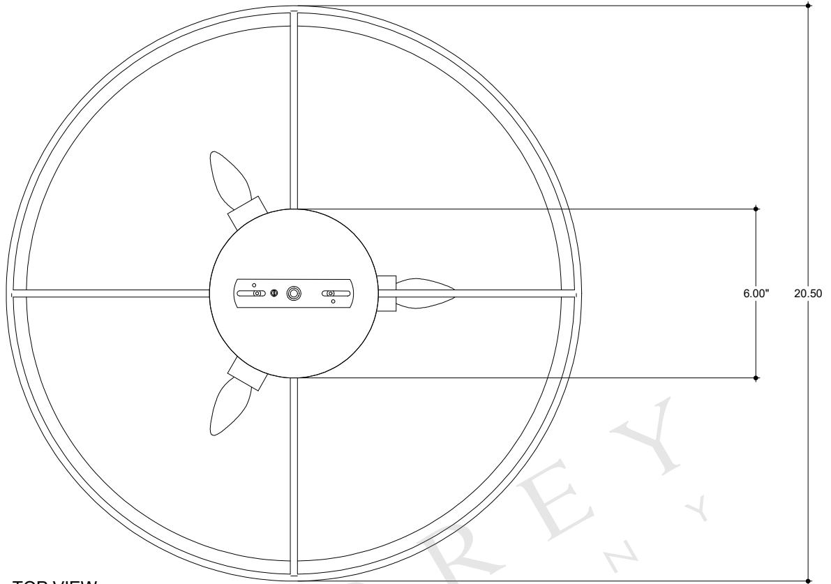
TOP VIEW
